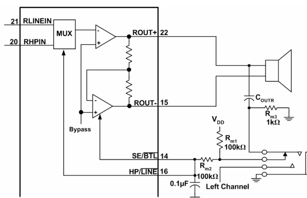
Figure 59. EUA5202 Resistor Divider Network Circuit
