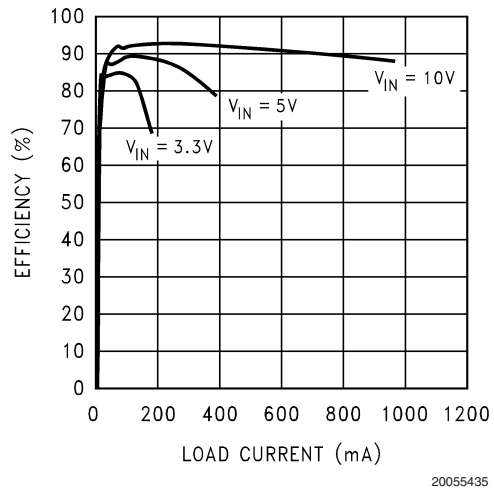
Efficiency vs Load ( V_{OUT} = 15V ) - "Y"
