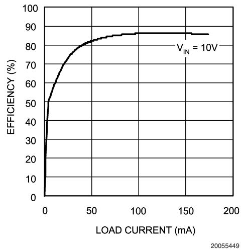
Efficiency vs Load ( V_{OUT} = 15V ) - "Y"
