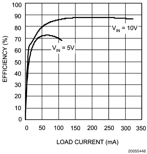
Efficiency vs Load Current ( V_{OUT} = 40V ) - "X"
