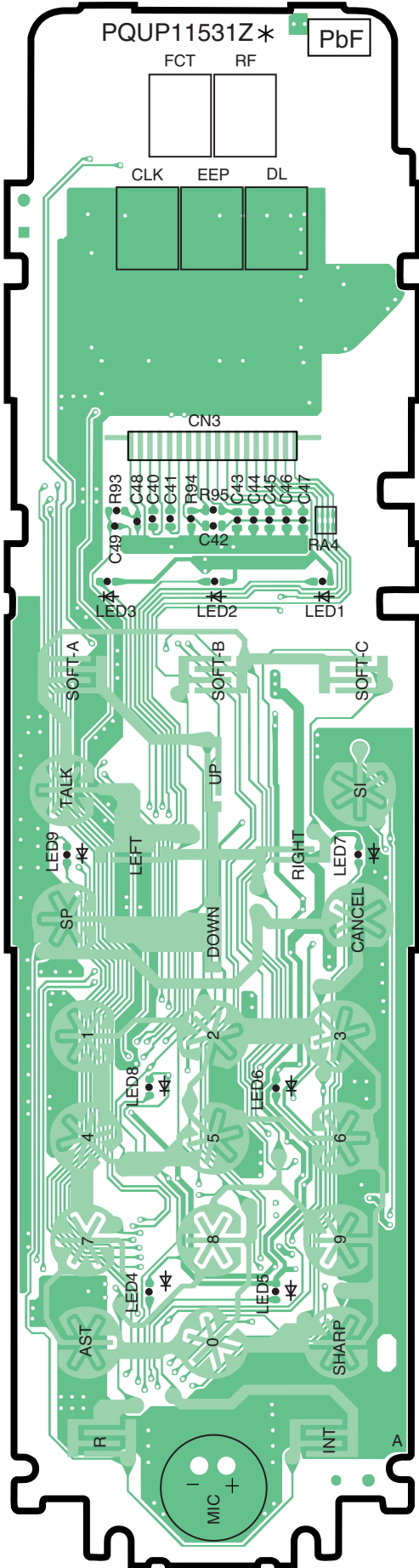
KX-TGA720 CIRCUIT BOARD (Handset (Flow Solder Side View))
