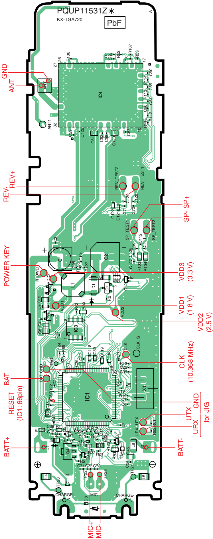
KX-TGA720 CIRCUIT BOARD (Handset (Component View))
