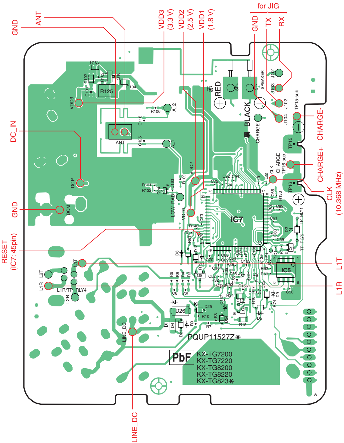
KX-TG7205/7206 CIRCUIT BOARD (Base Unit (Flow Solder Side View))
