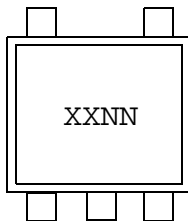
5-Lead SOT-23
