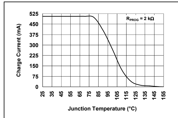
FIGURE 4-2: Thermal Regulation.
